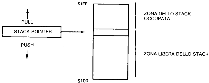
Figura 8.5 STACK e STACK POINTER
